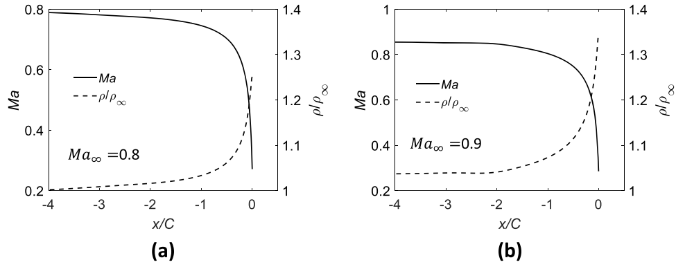
Fig. 11. Mach number and density ratio of the flow along the stagnation streamline for the flow past NACA0012 aerofoil at Re = 500 for far field Mach numbers (a) Ma_\infty = 0.8 and (b) Ma_\infty = 0.9 .
