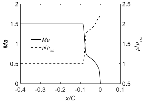
Fig. 14. Mach number and density ratio of the flow along the stagnation streamline for a supersonic flow across a NACA0012 aerofoil Ma_\infty = 1.5 , Re = 10^4 .
