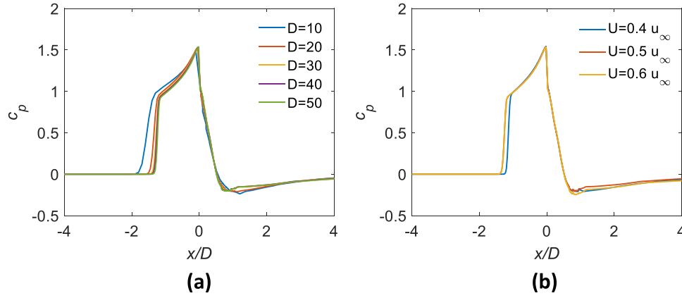
Fig. 5. Simulated pressure coefficients around the cylinder surface for a supersonic flow Ma_\infty = 1.6 , Re = 300 . (a) Various number of grid points along the diameter of cylinder and (b) various shifted velocity. x/D=0 position is at the cylindrical head.
