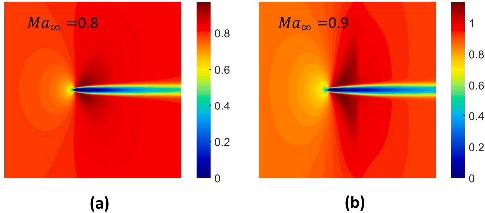
Fig. 9. Mach number distribution for transonic flow around a NACA0012 aerofoil at Re = 500 for far field Mach numbers (a) Ma_\infty = 0.8 and (b) Ma_\infty = 0.9 .
