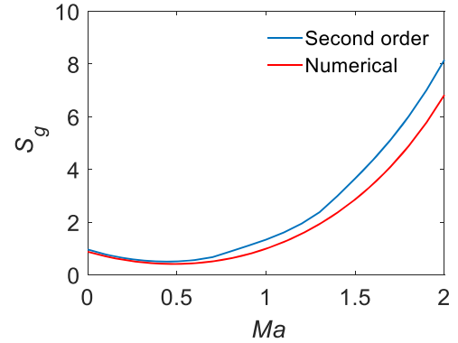
Fig. 2. Entropy function S_g = \sum_{i=1}^Q g_i \ln(g_i / W_i) estimated by second order approximation [20] and present numerical calculation as a function of Mach number.
