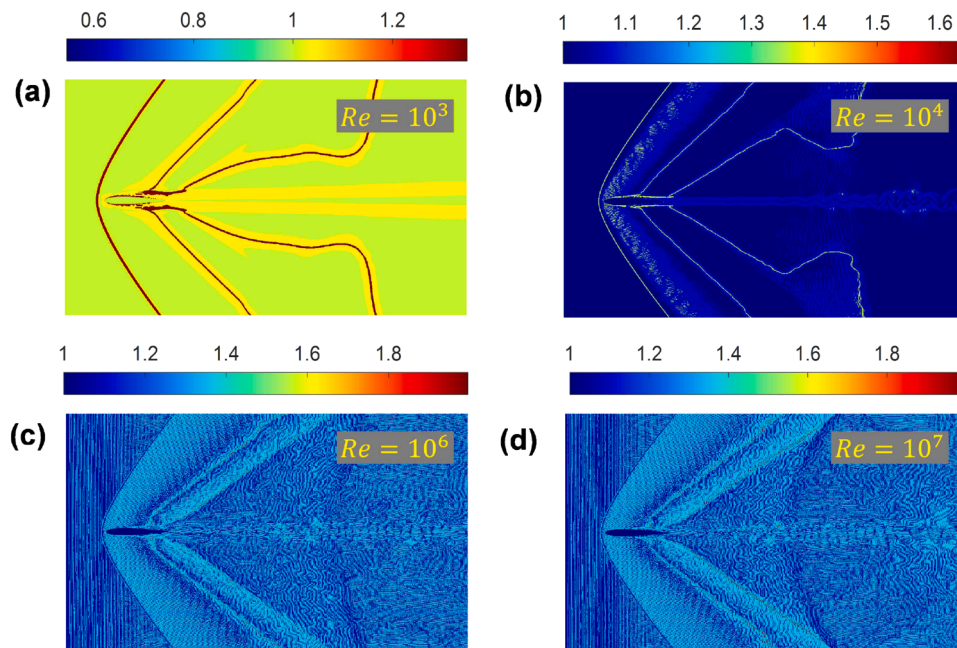
Fig. 16. Correction coefficients \sigma of supersonic flow past a NACA0012 aerofoil for Ma_\infty = 1.5 , C = 300 , varying Reynolds numbers Re (a) 10^3 , (b) 10^4 , (c) 10^6 and (d) 10^7 .
