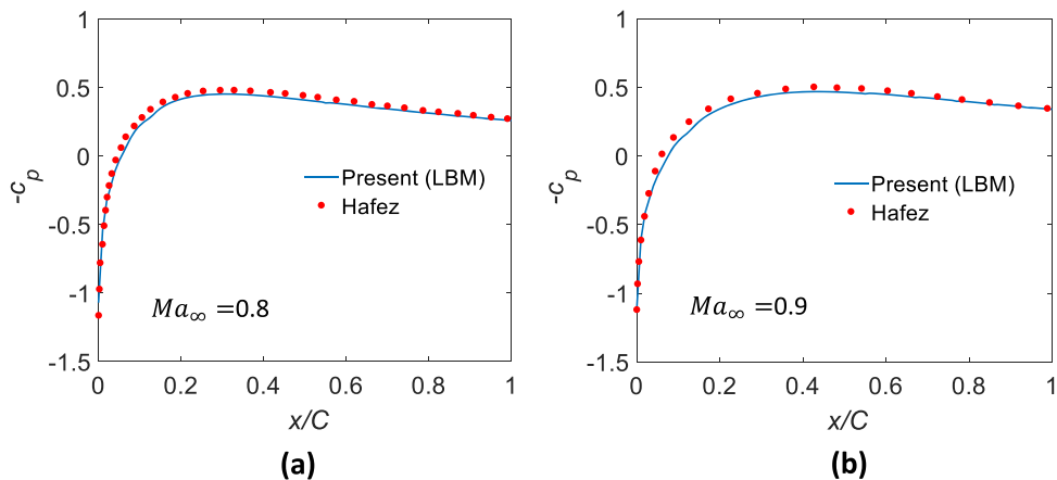
Fig. 10. Comparison of simulated pressure coefficient around NACA0012 aerofoil surface at Re = 500 for far field Mach numbers (a) Ma_\infty = 0.8 and (b) Ma_\infty = 0.9 , with Ref. [35].
