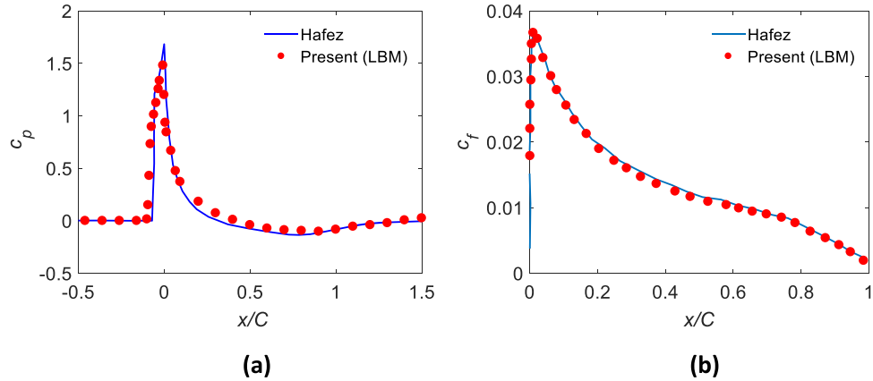
Fig. 13. Comparison of (a) simulated pressure coefficient and (b) skin friction coefficient around NACA0012 aerofoil surface ( Ma_\infty = 1.5 , Re = 10^4 ) using grid resolution C = 150 , with Ref. [36].
