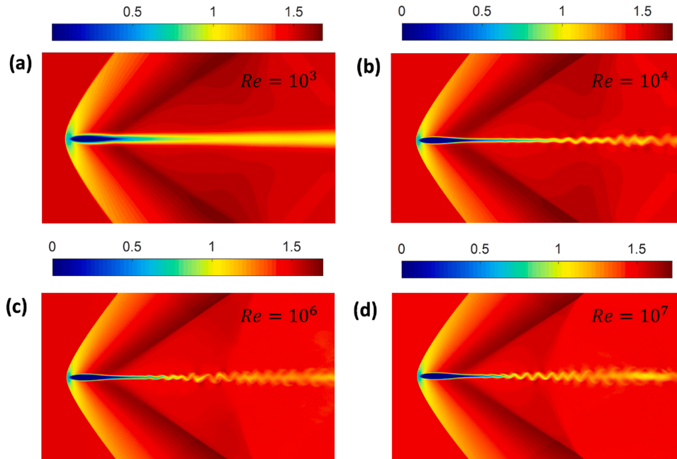
Fig. 15. Mach number fields for supersonic flow past a NACA0012 aerofoil for Ma_\infty = 1.5 , C = 300 , varying Reynolds numbers Re (a) 10^3 , (b) 10^4 , (c) 10^6 and (d) 10^7 .
