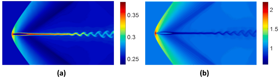
Fig. 12. (a) Temperature and (b) density fields for supersonic flow past a NACA0012 aerofoil with far-field flow of Ma_\infty = 1.5 , Re = 10^4 .
