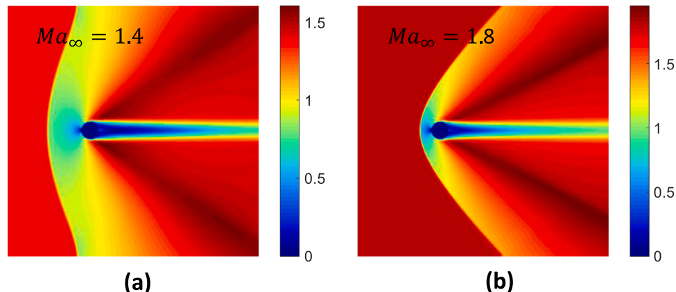
Fig. 7. Mach number field for supersonic flow around a cylinder for Re = 300 for far-field Mach numbers (a) Ma_\infty = 1.4 and (b) Ma_\infty = 1.8 .
