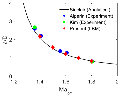
Fig. 8. Comparison of modelled shock stand-off distance \delta/D with respect to far field Mach number Ma_\infty against reported experimental [33,34] and analytical solutions [33].
