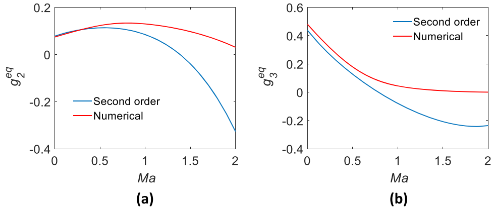
Fig. 1. Equilibrium populations estimated by second order approximation [20] and present numerical calculation as a function of Mach number. (a) g_2^{eq} and (b) g_3^{eq} .
