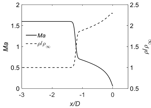
Fig. 6. Mach number and density ratio of the flow along the stagnation streamline for a supersonic flow across a circular cylinder Ma_\infty = 1.6 , Re = 300 .
