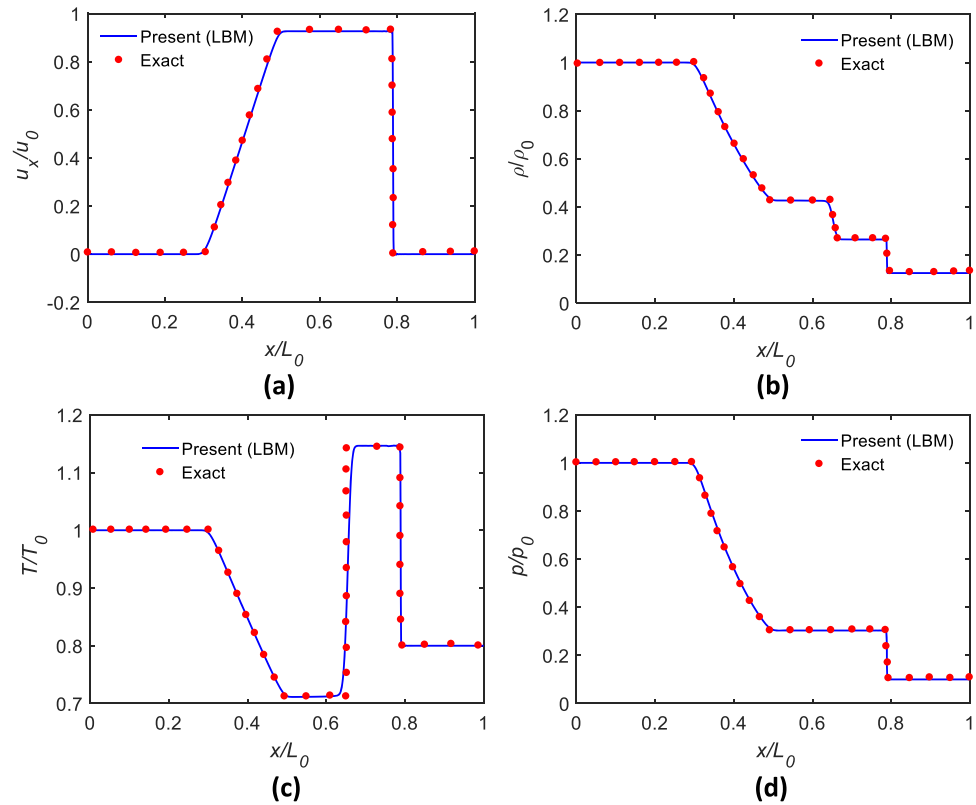
Fig. 4. Comparison of non-dimensional gas properties along the Sod shock tube between present LBM result and exact solution [32]. (a) Velocity, (b) density, (c) temperature and (d) pressure.
