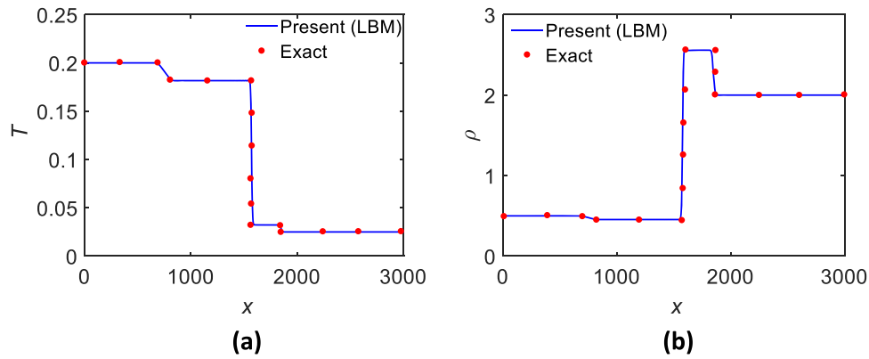
Fig. 3. Comparison of gas properties along the Sod shock tube between present LBM result and exact solution [20]. (a) Temperature and (b) Density.
